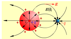
Figure 3: 矢量场可视化
