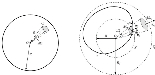
Figure 5: 球面和闭曲面上面元的立体角
