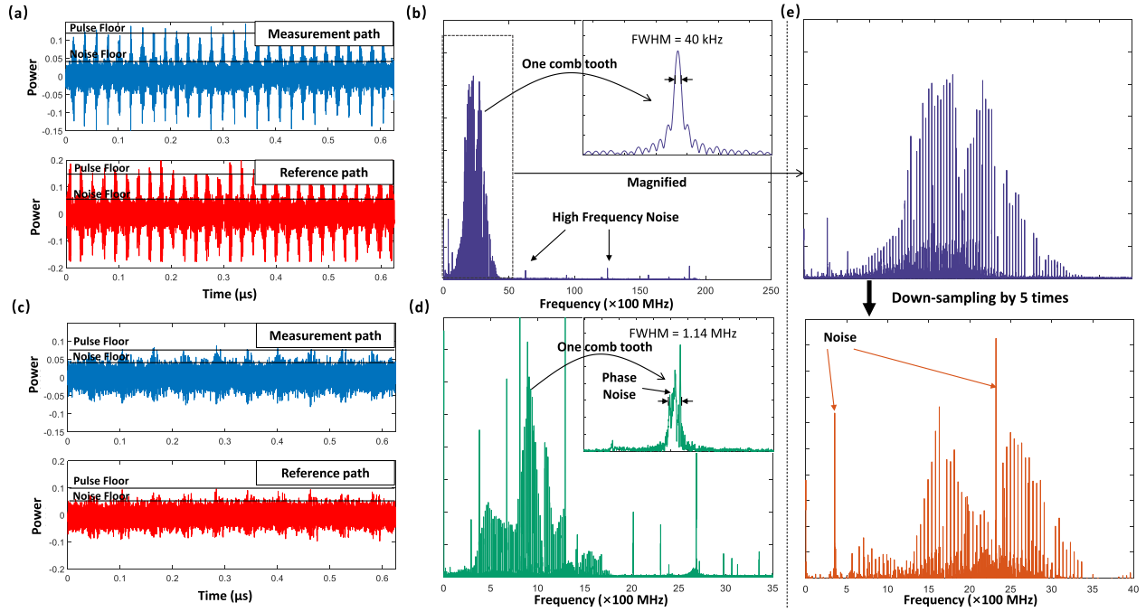
Fig. 5. Comparison between coherent dual-comb ranging and free-running dual-comb ranging. (a) 0.625 \mu s of recorded signals when using two coherent microcombs. The signal-to-noise rate is about 4 in both paths. (b) The Fourier transform of signal in (a). The FWHM is 40 kHz. (c) 0.625 \mu s of recorded signals when using two free running microcombs. The signal-to-noise rate is lower than 2 in both paths. (d) The Fourier transform of signal in the measurement path in (c) (only 0 - 2 GHz shown). The full width at half maximum (FWHM) is 1.14 MHz. (e) Comparison between the Fourier transform of the original data (with sampling rate at 50 GSa/s) and the data down-sampled by 5 times. Several high-frequency noise with higher frequencies in the RF spectrum appears at lower frequencies after down-sampling.
